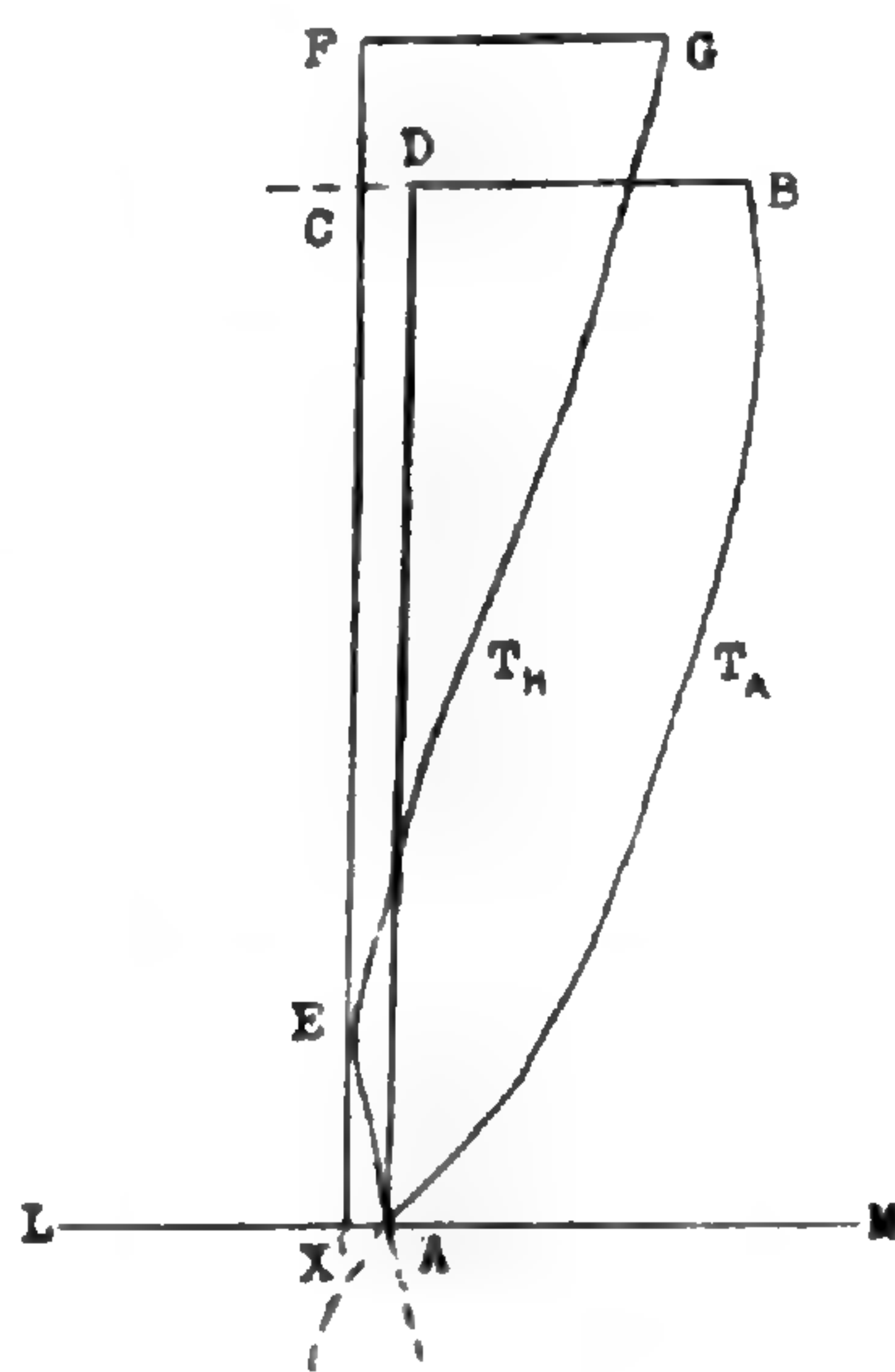
Fig. 4. Method of determining the "degree-hours."
